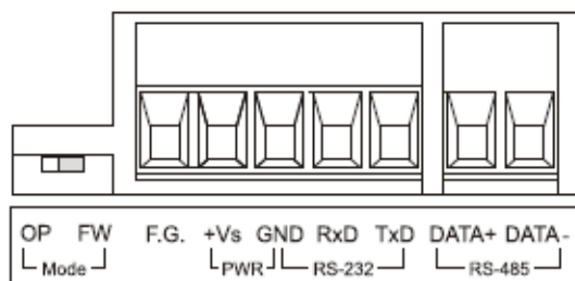
Figure 2-3 Communication terminal
